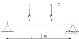
JÁCENA PRINCIPAL
